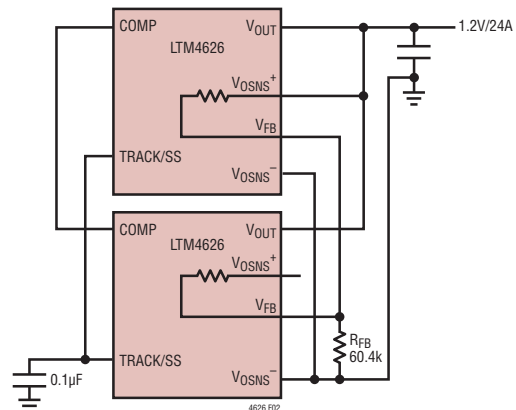
Figure 2. 2-Phase Parallel Configurations
