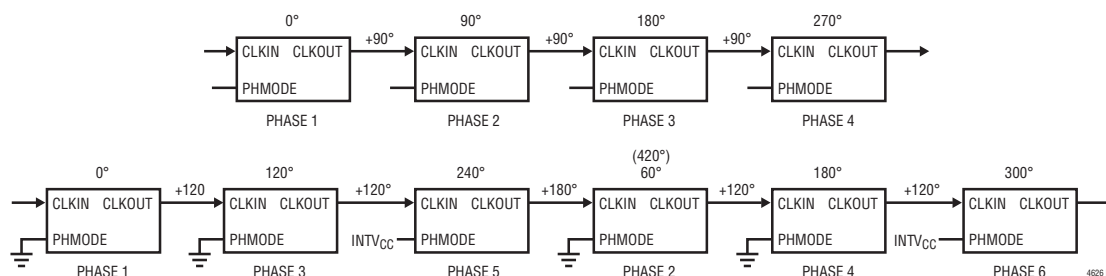
Figure 3. 4-Phase, 6-Phase Operation
