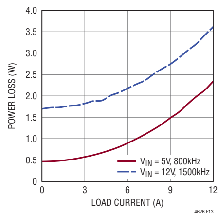
Figure 13. Power Loss at 3.3V Output
