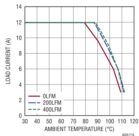
Figure 16. 12V to 1V Derating Curve, No Heat Sink
